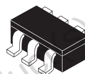
SOT323-6L STDD15-xxS
